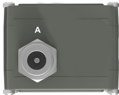
Connector A (standard) Type: N female, (option F female or SMA female) Functions: L-Band out, DC in, External 10 MHz in
