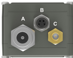
Connector B (optional) Type: M8 female, 4 pin, A-coded Functions: Alarm and M&C
