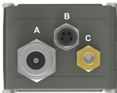
Connector B (optional) Type: M8 female, 4 pin, A-coded Functions: Alarm and M&C
