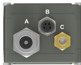
LNB connectors (optional)
