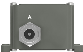
Connector A (standard) Type: N female (option F female or SMA female) Functions: L-Band out, DC in, External 10 MHz in
