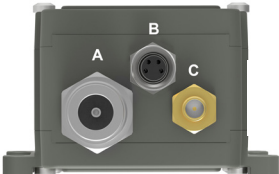
Connector B (optional) Type: M8 female, 4 pin, A-coded Functions: Alarm and M&C
