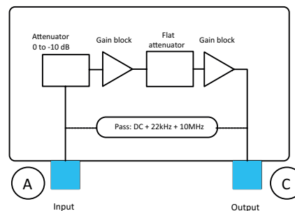
Flat 24 dB gain model
