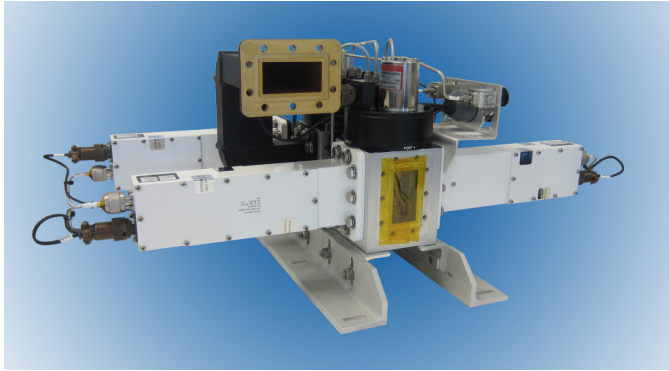
Typical C-Band 1:2 LNA Plate Assembly
