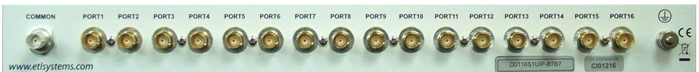
Rear View of Model D0116S1UIP with 75 ohm BNC connectors
